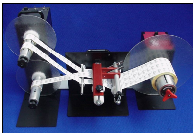
Complete TWIN-SLIT-100 Package
